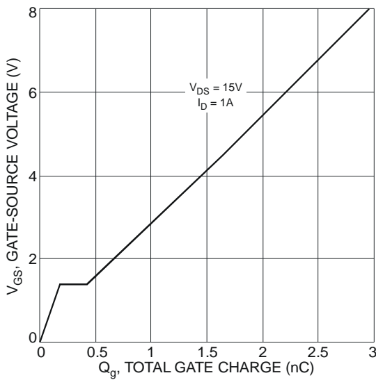
Fig. 11 Gate-Charge Characteristics
